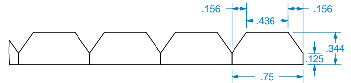
DETAIL A SCALE 1:1
