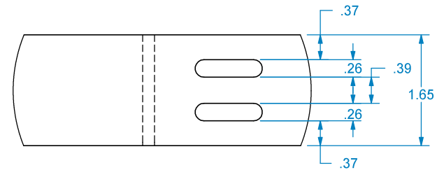
DETAIL A SCALE 1 : 2
