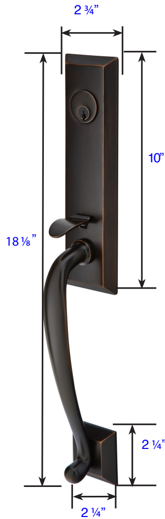
Adams Style Part # 4414/4424
