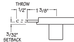
CB-241 TYPE 241 CYLINDER BODY
