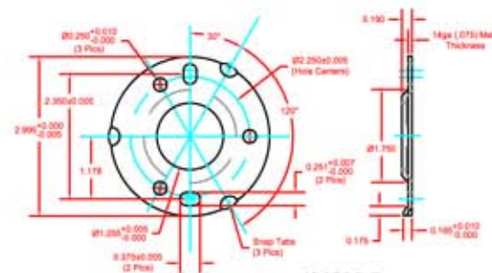
IOCR5-B-Flange Detail
