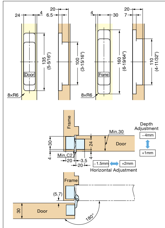
Bore Dimensions
